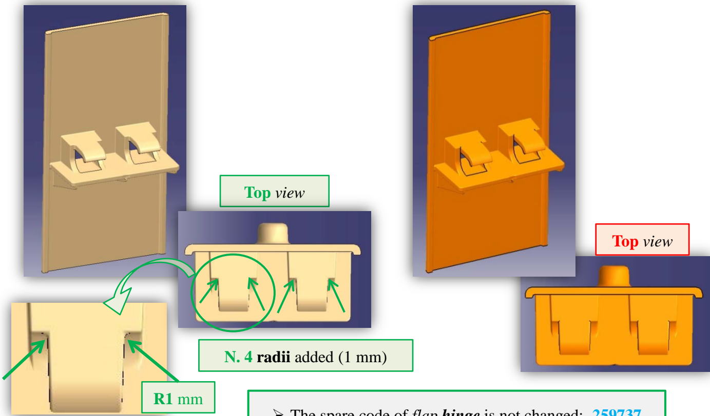
Pre - modification flap hinge
