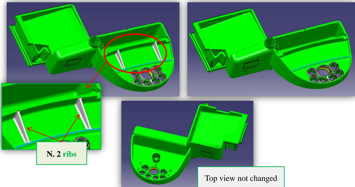
Modified nozzles support
