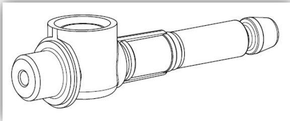
Radius of the gasket seat increased
