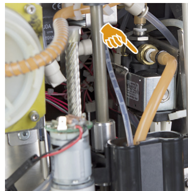
Installation of switching valve from 1/4/2017
