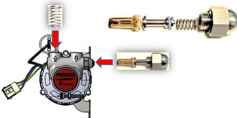
Figure 2: Installation of repair set
