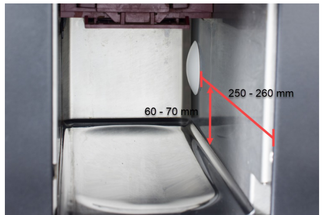
Figure 2: ABS buffer glued into the brewing shaft
