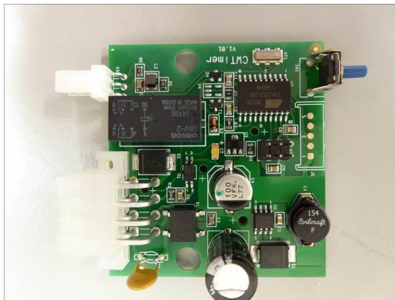
Blue switch PCB (CW timer V1,01)
