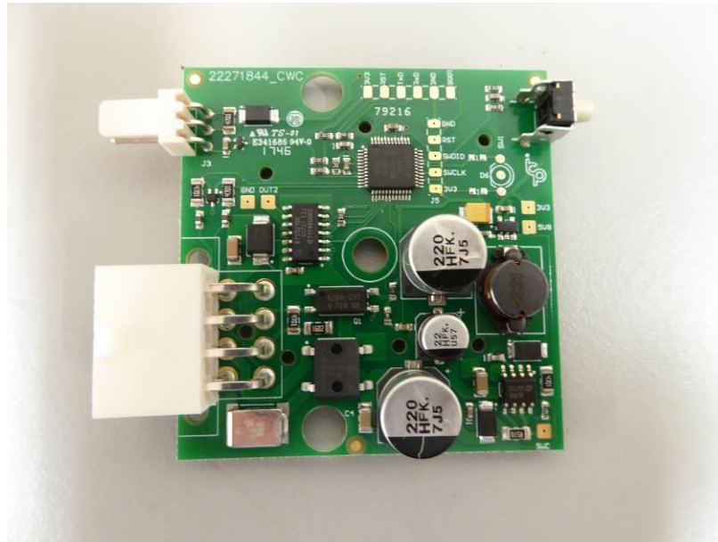
White switch PCB (22271844_CWC)
