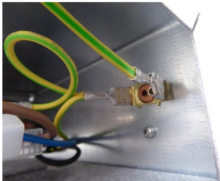
Earth connection
